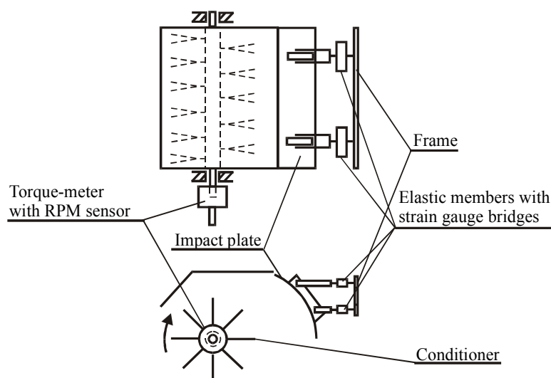
Fig. 1. Equipment for material feed rate measurement
