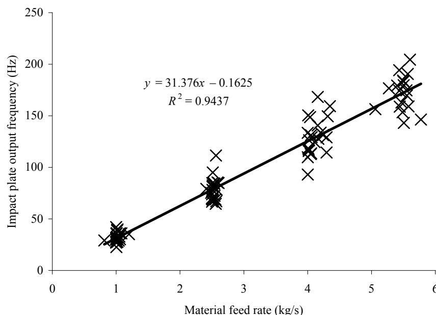
Fig. 4. Measured values from impact plate measurement
