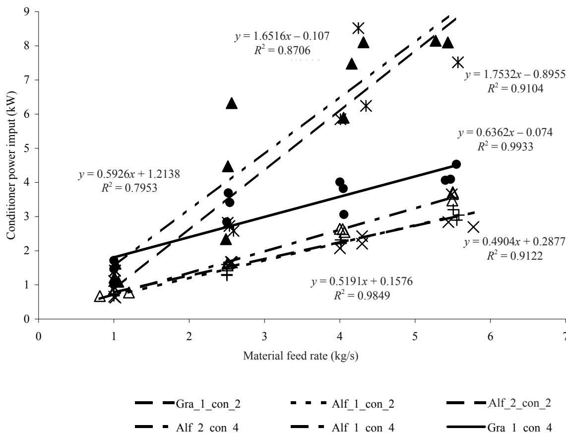
Fig. 3. Graphic comparison of tested files from torque-meter measurement
