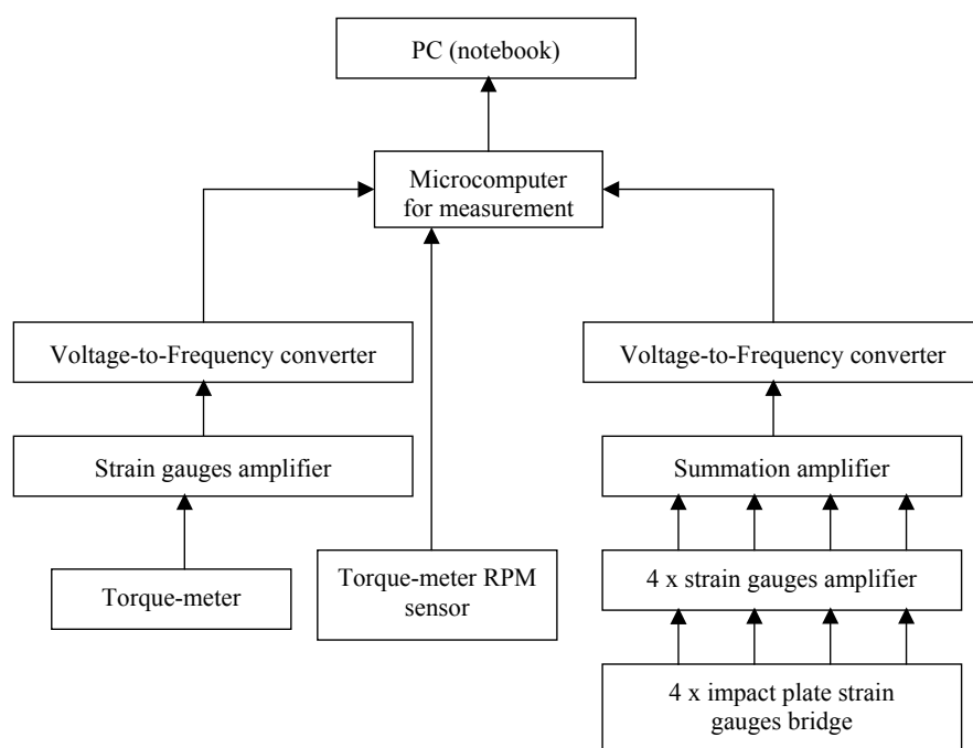
Fig. 2. Block diagram of electronic apparatus arrangement for material feed rate measurement
