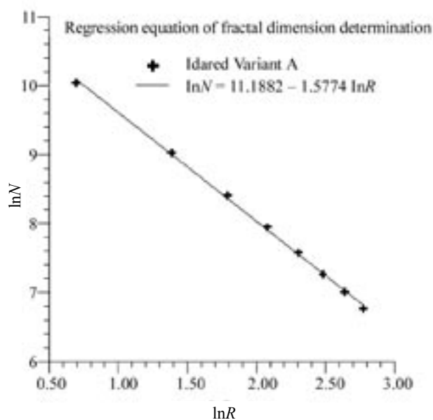
Fig. 3. Determination of fractal dimension as the slope of the line by method of regression
