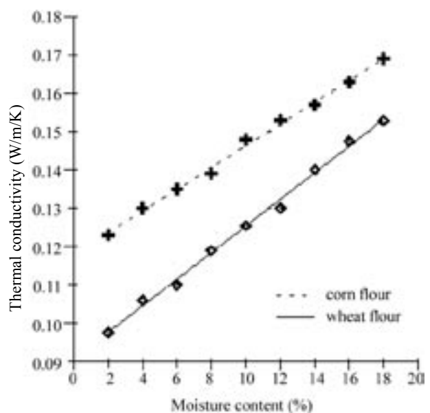
Fig. 1. Relations of thermal conductivity \lambda to moisture content \omega for corn flour and wheat flour
