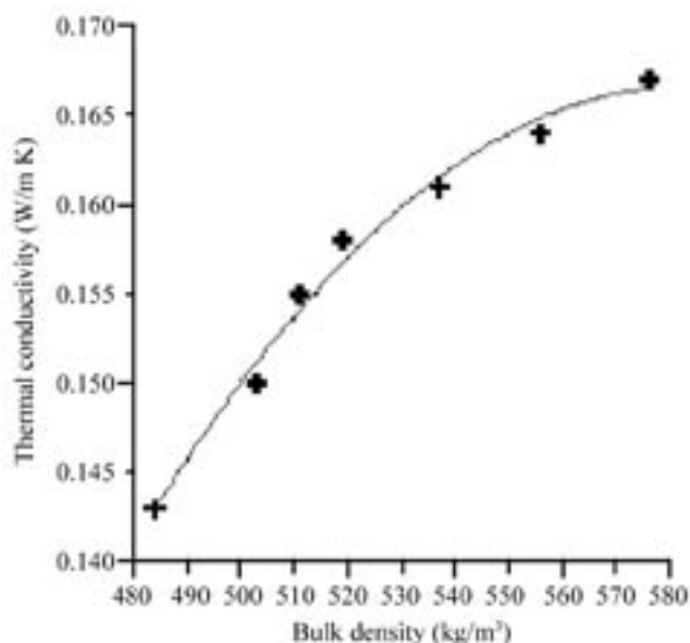
Fig. 5. Relation of thermal conductivity \lambda to bulk density \rho_s – wheat flour
