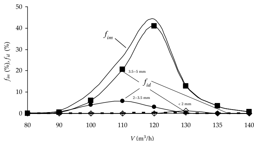
Figure 2. The dependence of relative weight frequencies f_{im} (%) and f_{id} (%) on the airflow quantity V (m³/h)
