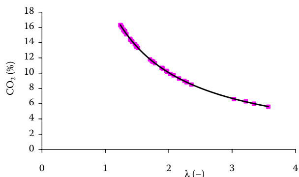
Figure 6. Dependence of CO 2 emissions on excess air factor \lambda at combustion of briquette timothy grass hay
