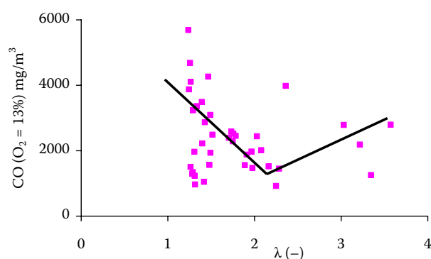
Figure 7. Dependence of CO emissions on excess air factor \lambda at combustion of briquette timothy grass hay
