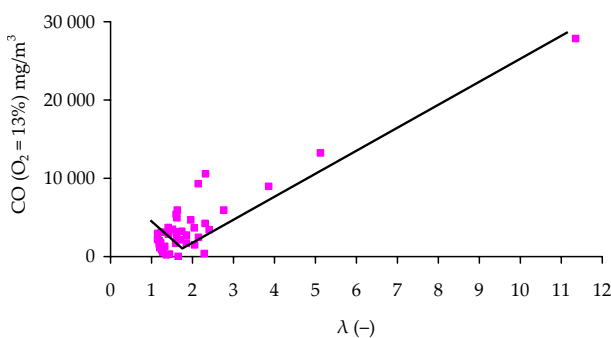
Figure 9. Dependence of CO emissions on excess air factor \lambda at briquette combustion from mixture of meadow hay with 25% m/m of brown coal
