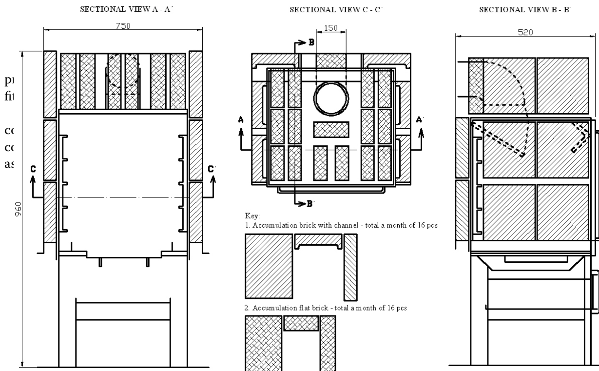
Figure 1. Optimized layout of accumulation bricks of verified combustion stove SK-2 RETAP
