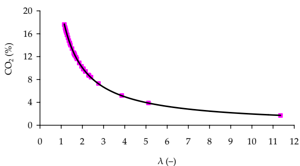
Figure 8. Dependence of CO 2 emissions on excess air factor \lambda at briquette combustion from mixture of meadow hay with 25% m/m of brown coal
