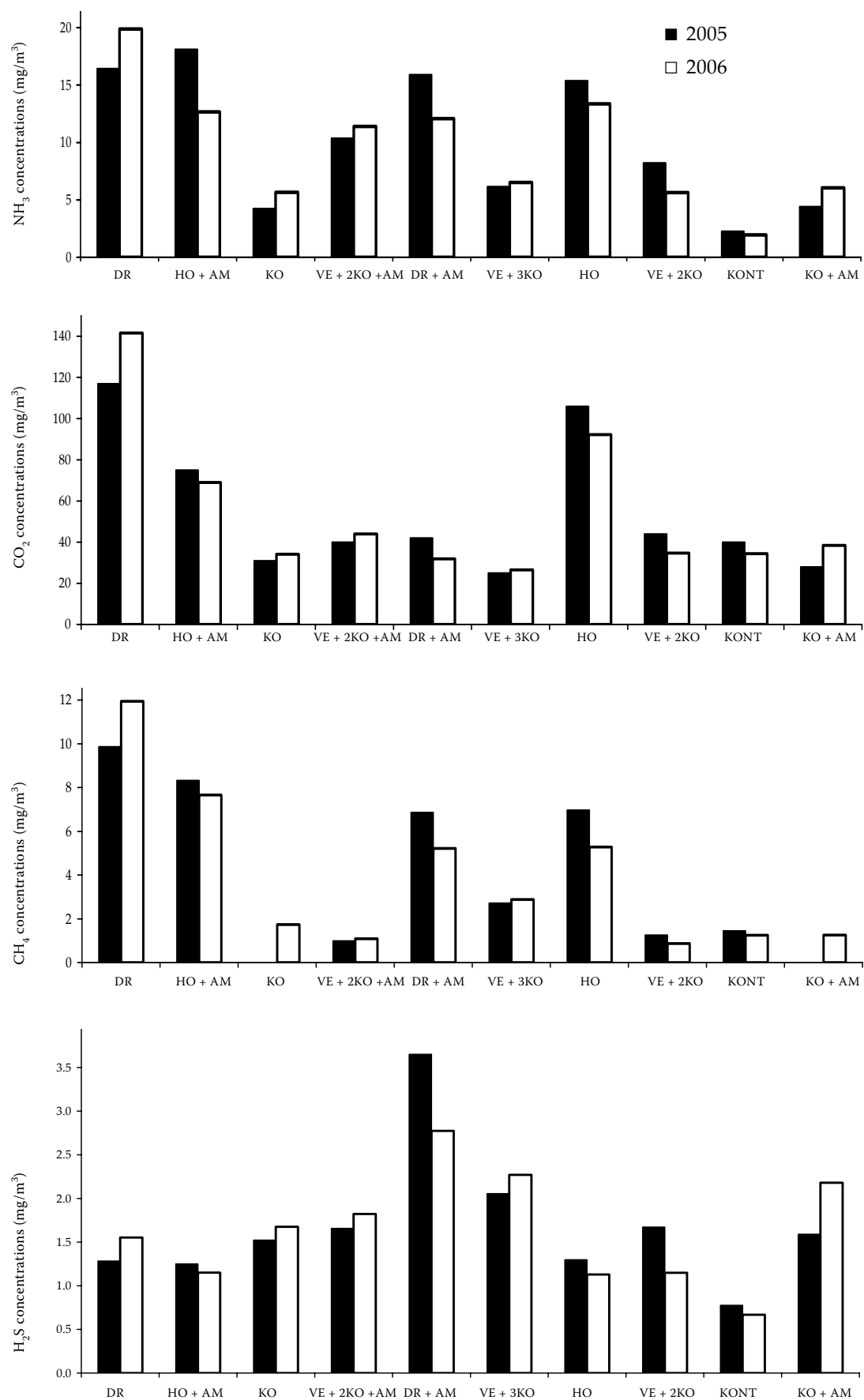
Figure 1. Average NH 3 , CO 2 , CH 4 , and H 2 S concentrations – trial No. 1 and 2
