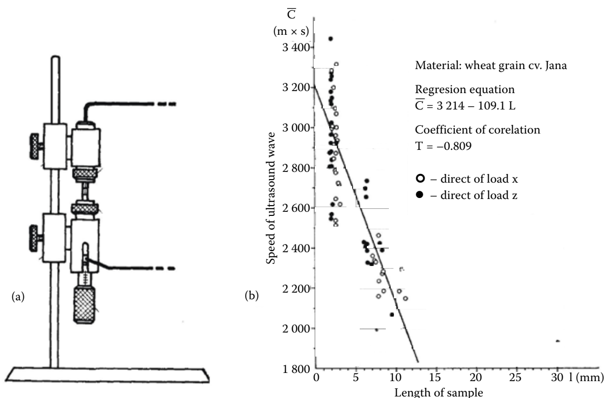
Figure 4. Diagram of the mechanical part of the equipment used to measure the speed of ultrasound waves in grain endosperm (a), and the values of the speed of ultrasound wave front in the endosperm of wheat and the course of its regression dependence on the height of sample column (b)
