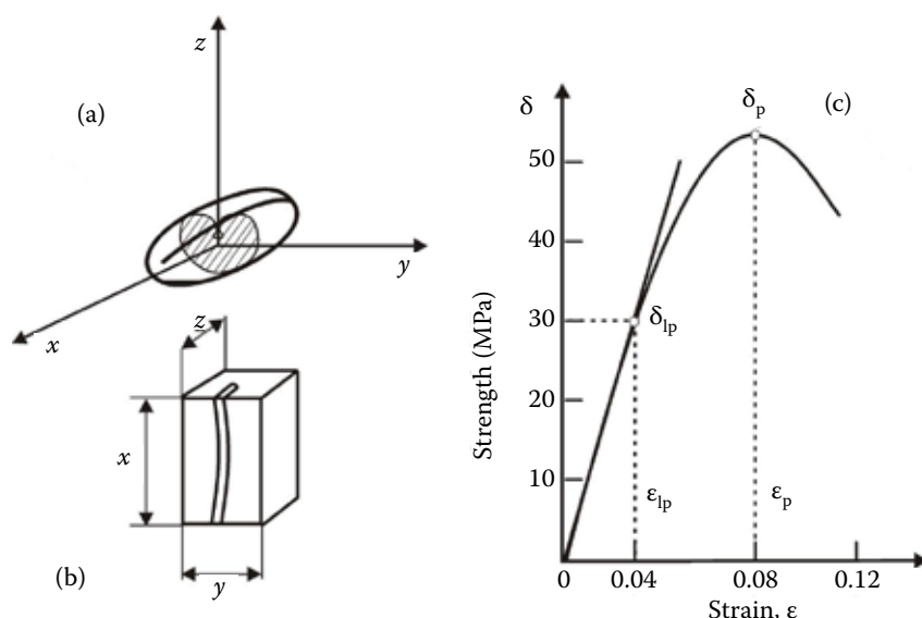
Figure 3. Wheat grain spatial orientation (a), endosperm section shape (b), and characteristic curve with parameters recorded by Instron machine (c)
