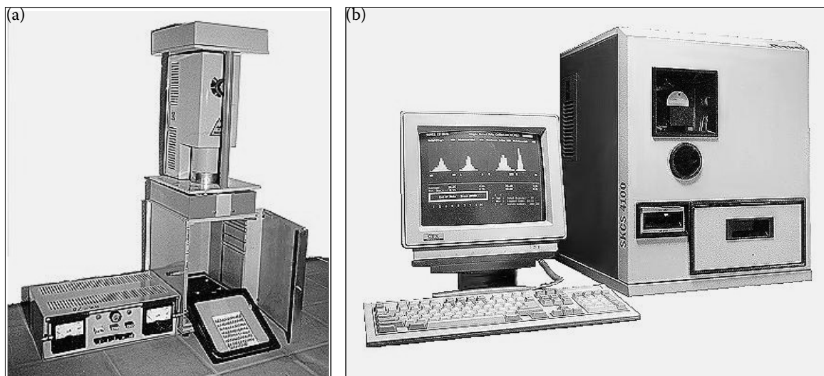
Figure 2. View of the X-ray apparatus (a), and the SKCS (b)
