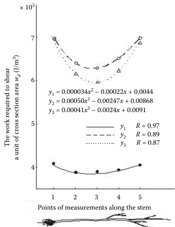
Figure 7. Distribution of the values of the shearing energy per stem cross-section area unit in dynamic test along the stem of Jupiter rape in successive phenophases ( y_1, y_2, y_3 – regression curve, y_1 – complete silique filling, y_2 – technical ripeness, y_3 – full ripeness)
