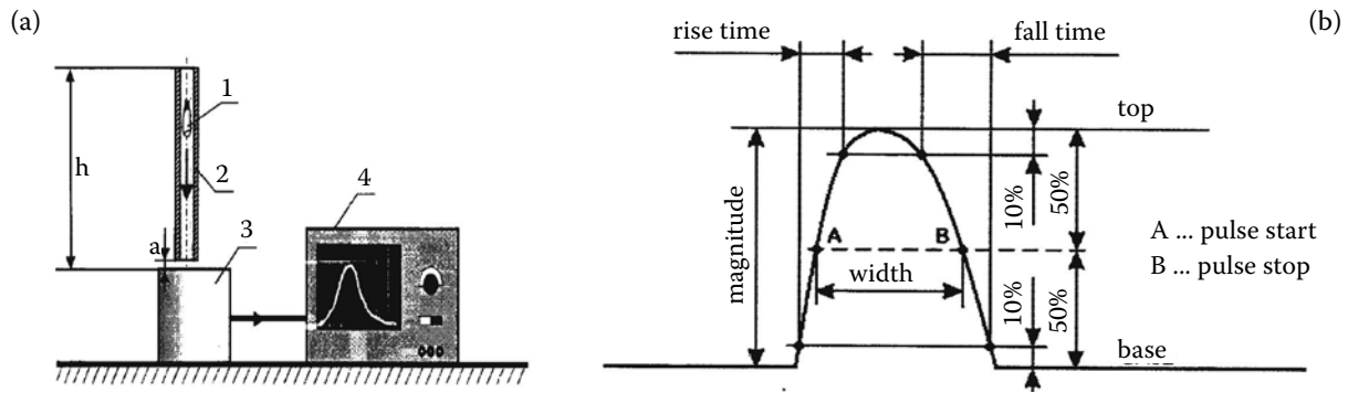
Figure 6. Scheme of the used apparatus (a): 1 – barley kernel, 2 – glass tube, 3 – force transducer, 4 – digital oscilloscope (DSO); and graphic presentation of the pulse parameters and their geometric sense (b)
