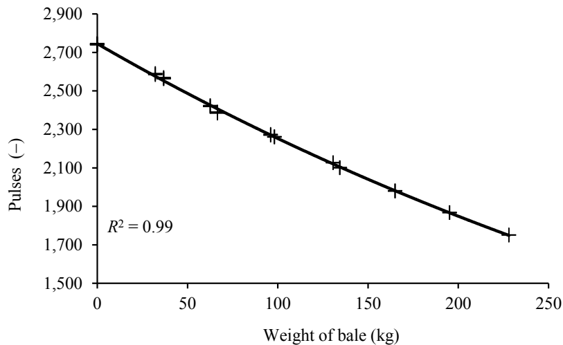
Fig. 3. Dependence of pulses count on weight increment of a bale
