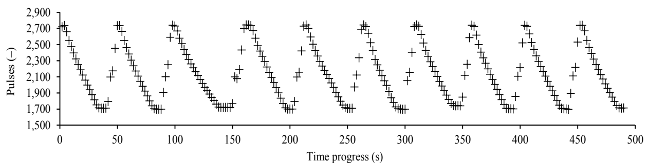
Fig. 4. Adapted measured values – number of pulses in time (during real harvest)
