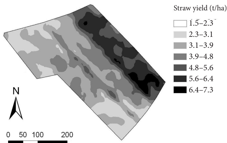
Fig. 6. Yield map of straw (t/ha)
