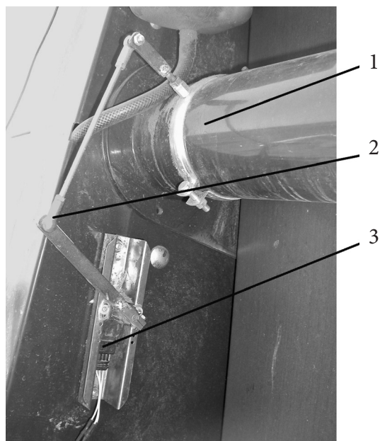
Fig. 1. Technical description of potentiometer position 1 – belt tension roller mechanism, 2 – connecting rod, 3 – potentiometer
