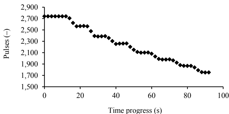
Fig. 2. Course of data record during discontinuous straw row pressing
