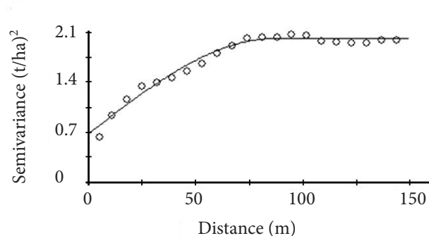
Fig. 5. Variogram of straw yield (t/ha)
