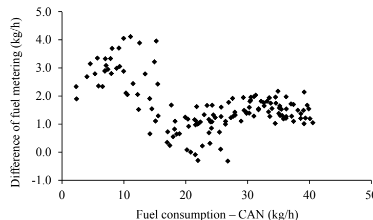
Fig. 6. Difference of values of direct and indirect fuel consumption metering (Claas Axion 850 Cebis)
