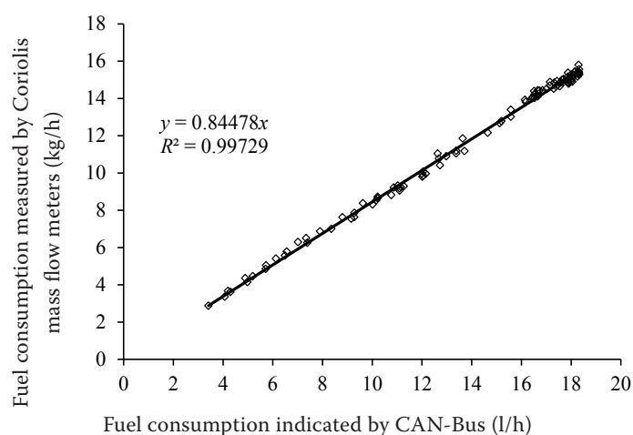
Fig. 17. Dependence of fuel consumption detected by the Coriolis flow meter on CAN fuel consumption of John Deere 5080RN tractor
