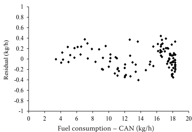
Fig. 18. Residual deviations from the calculated regression line (John Deere 5080RN)
