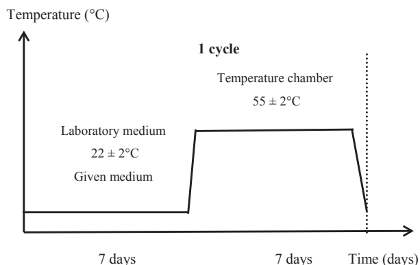
Fig. 1. Transformational diagram of the bonded joints testing at the exposure to different media
