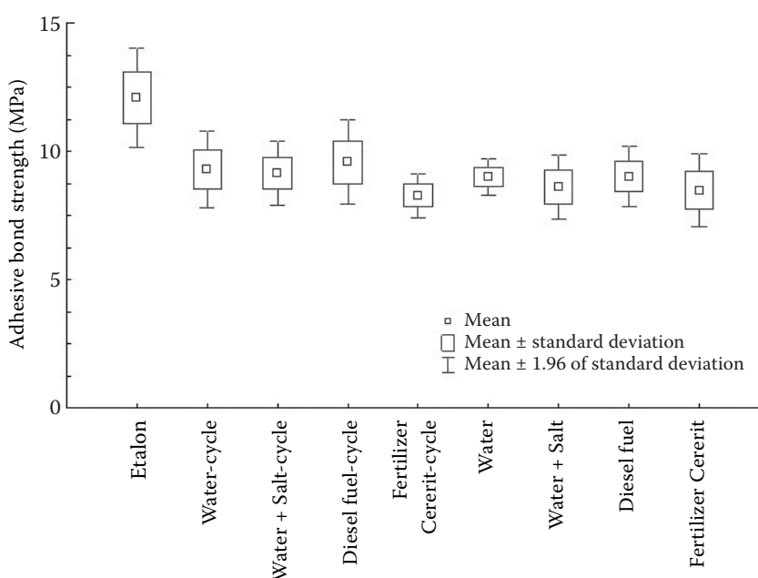
Fig. 9. Influence of degradation medium on the bonded joint strength
