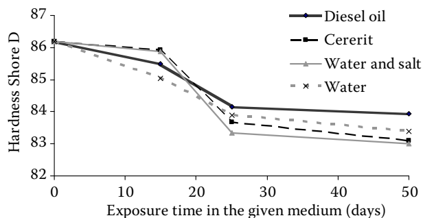
Fig. 7. Influence of degradation medium on the Shore D adhesive hardness
