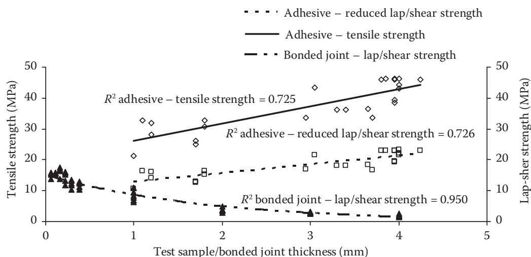
Fig. 2. Influence of tested sample and bonded joint thickness on the strength
