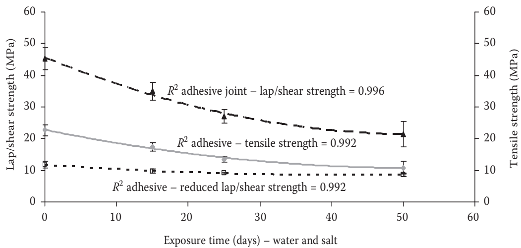
Fig. 4. Influence of degradation medium on the bonded joint and adhesive strength
