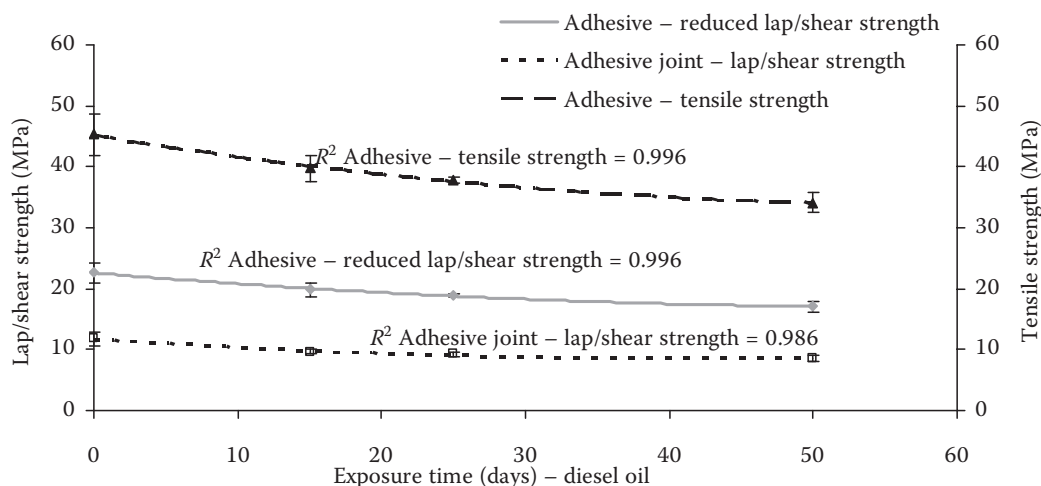
Fig. 6. Influence of degradation medium on the bonded joint and adhesive strength
