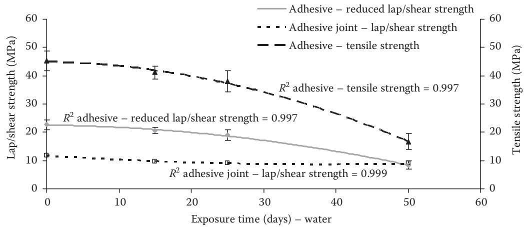
Fig. 3. Influence of degradation medium on the bonded joint and adhesive strength
