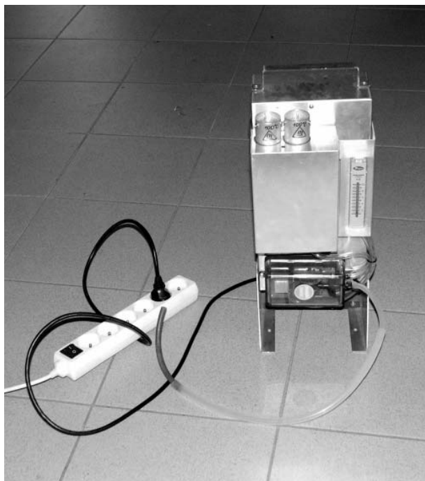
Fig. 4. Ozone measuring equipment APOA 350 E in the diagnostic vehicle
