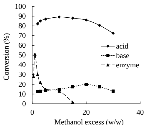
Fig. 1. Relation between methanol excess and conversion in rendering plant fat transesterification
