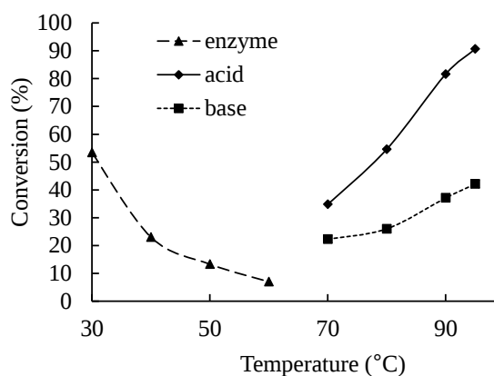
Fig. 4. Influence of reaction temperature in rendering plant fat transesterification
