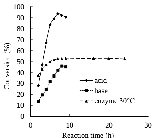
Fig. 5. Influence of reaction time in rendering plant fat transesterification
