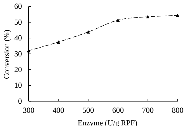
Fig. 3. Relation between enzyme dose and conversion in rendering plant fat transesterification
