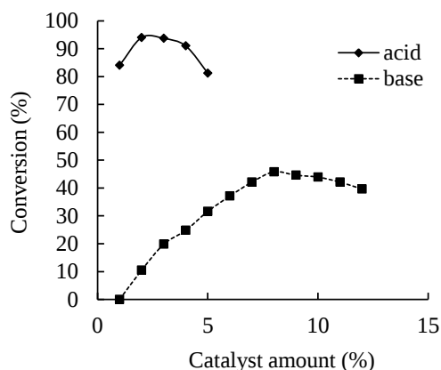
Fig. 2. Relation between catalyst (acid or base) doses and conversion in rendering plant fat transesterification
