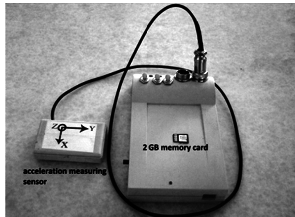
Fig. 3. Tractor seat base vibration measuring apparatus
