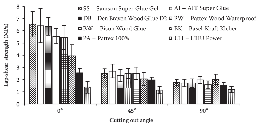
Fig. 2. Relationship between the tensile lap-shear strength and the cutting out angle; standard
